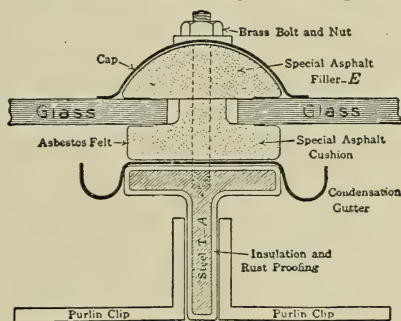
FIG. 150.—Pre-formed Washers for Sky-lights.
